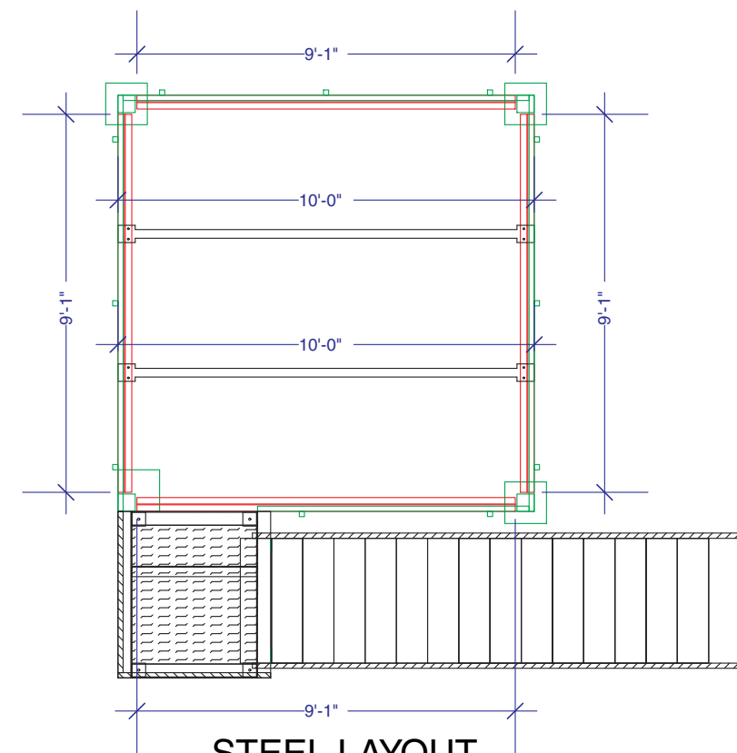
STEEL LAYOUT
