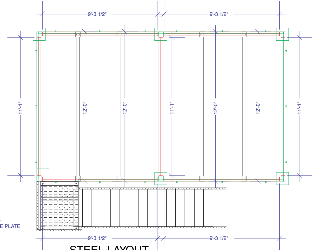
STEEL LAYOUT
