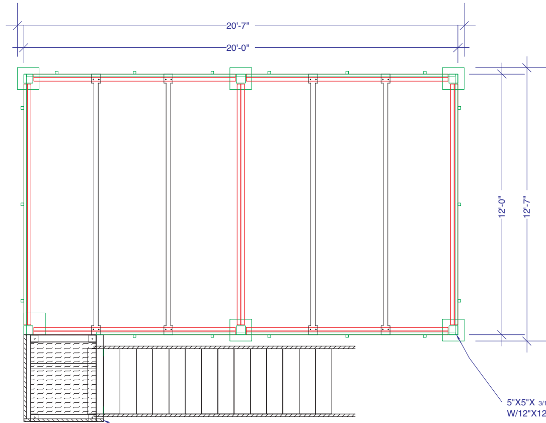
FLOOR PLAN
